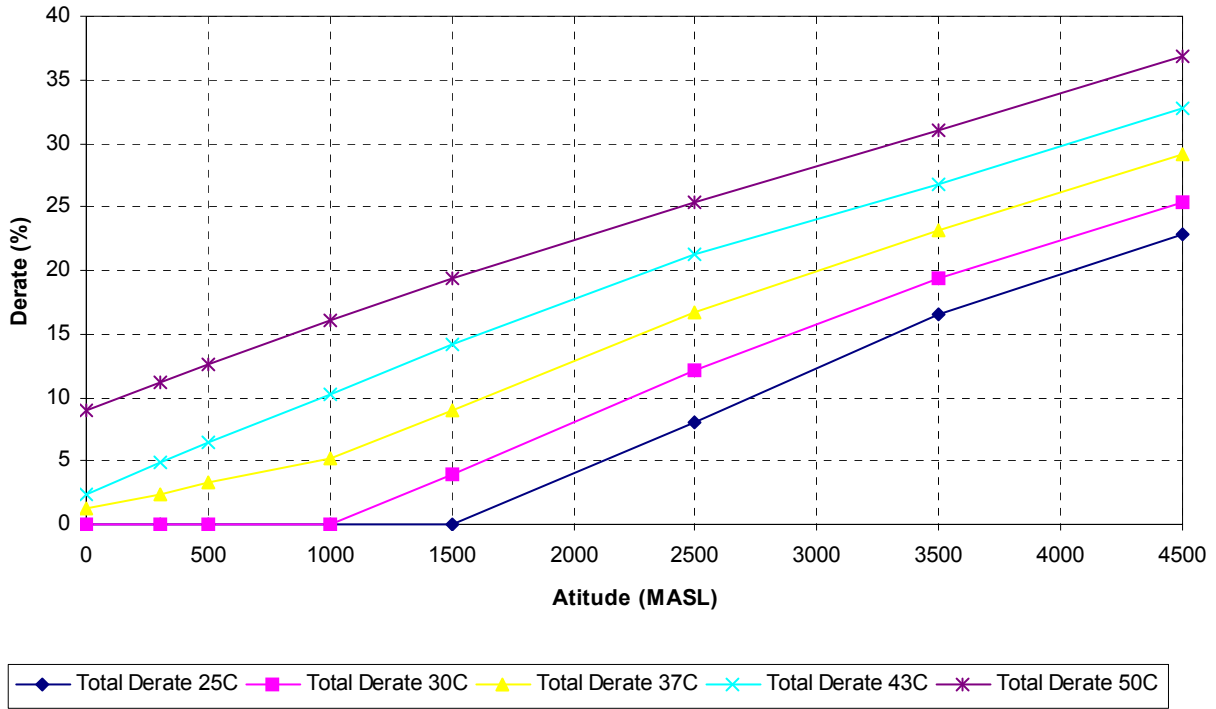
Derate Chart 2806-E18 700 kVA Low BSFC
