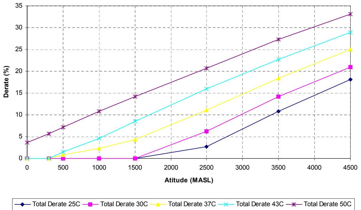
Derate Chart 2806-E18 660 kVA Low BSFC
