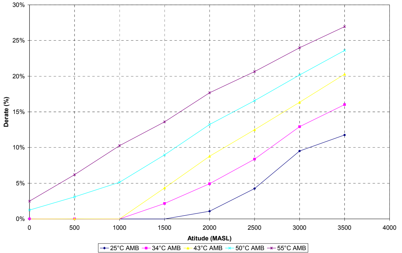
Derate Chart 2206A-E13 TAG3 450 kVA Low BSFC
