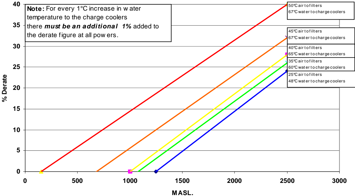
4016-61TRG3 1500 rev/min Non-Ems derate for high air temperature. And/or elevated altitude from ISO 3046 standard conditions. June 2010
