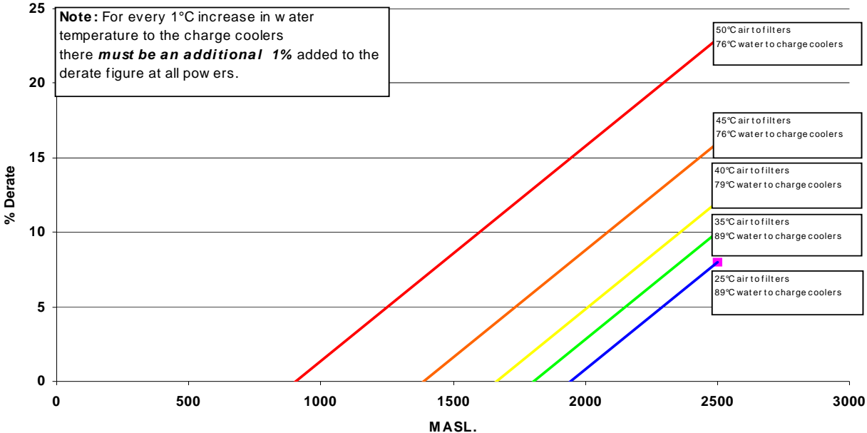
4016-61TRG2 1500 rev/m in Non-Em s derate for high air temperature. And/or elevated altitude from ISO 3046 standard conditions. June 2010
