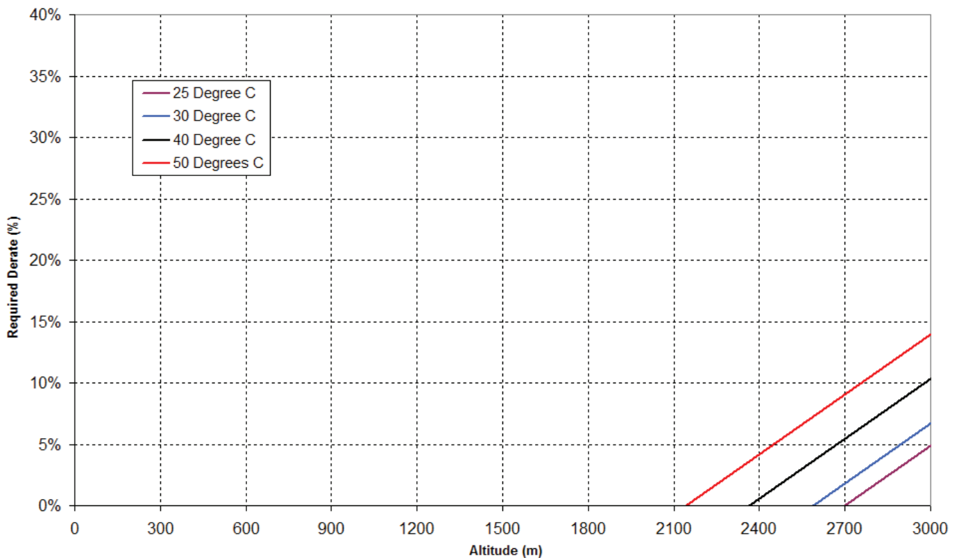
1106A-70TAG2 60Hz Prime Derate Chart
