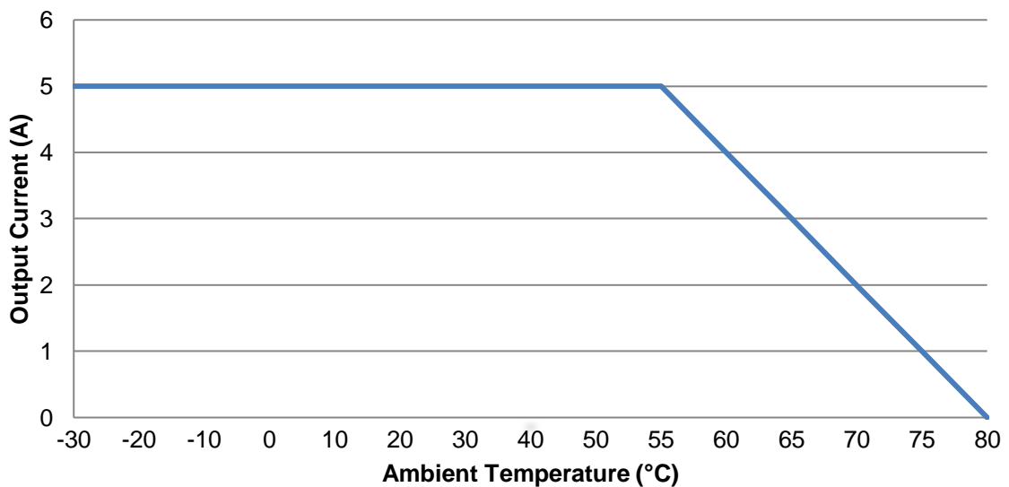
DSE9481 (MKII) Temperature Derate Curve 90 V < Vin < 305 V
